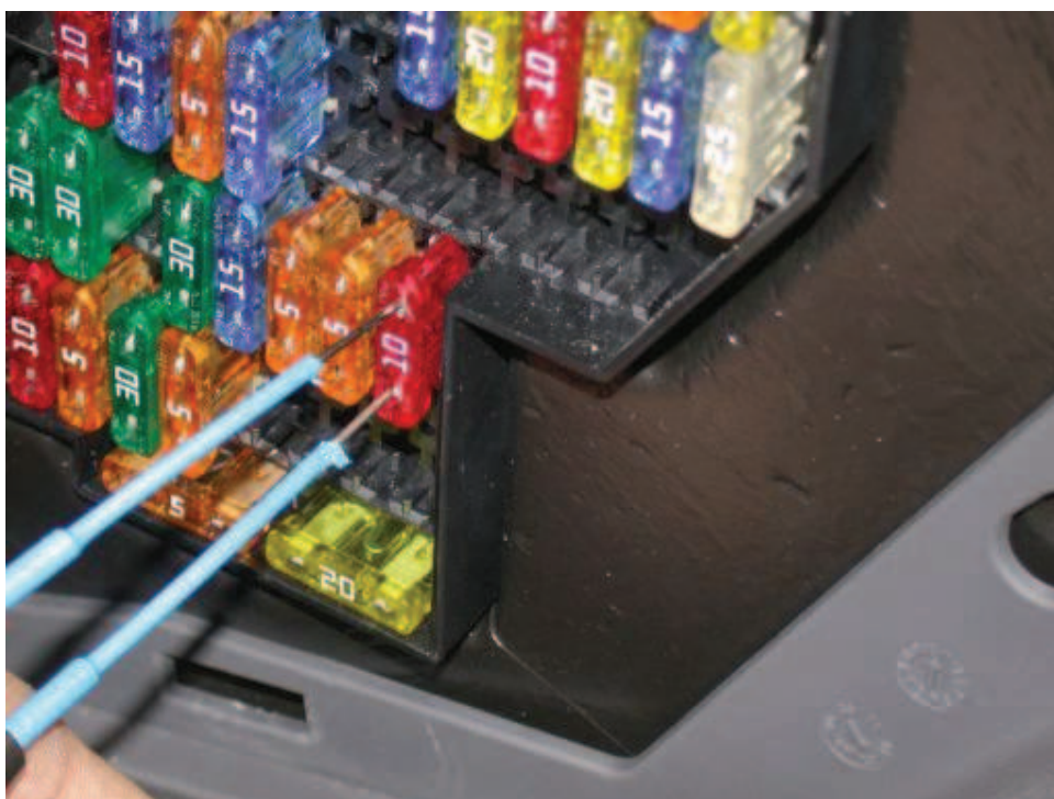
Illustration 1: Current measurement via fuse
