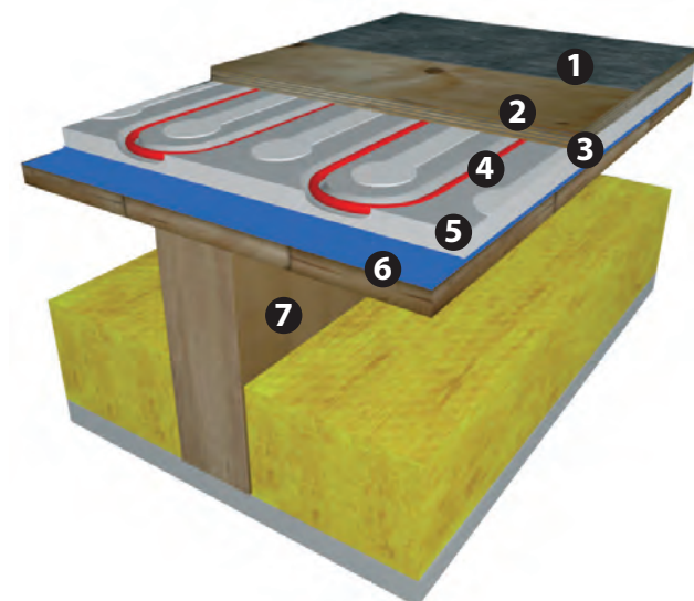
Fig. 22. Floor heating with DEVIcell™ on existing wooden floors
